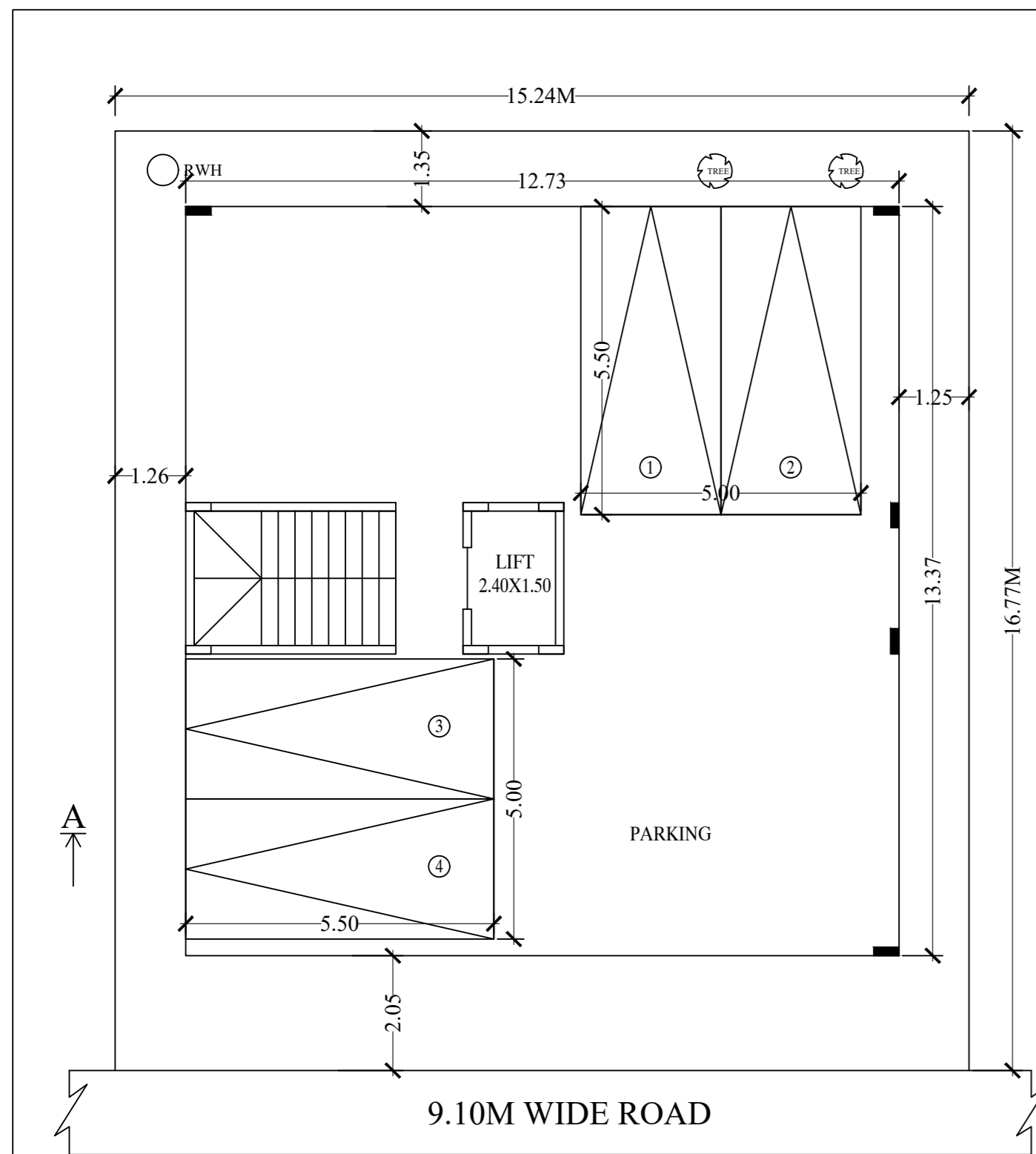
PROPOSED STILT FLOOR PLAN
